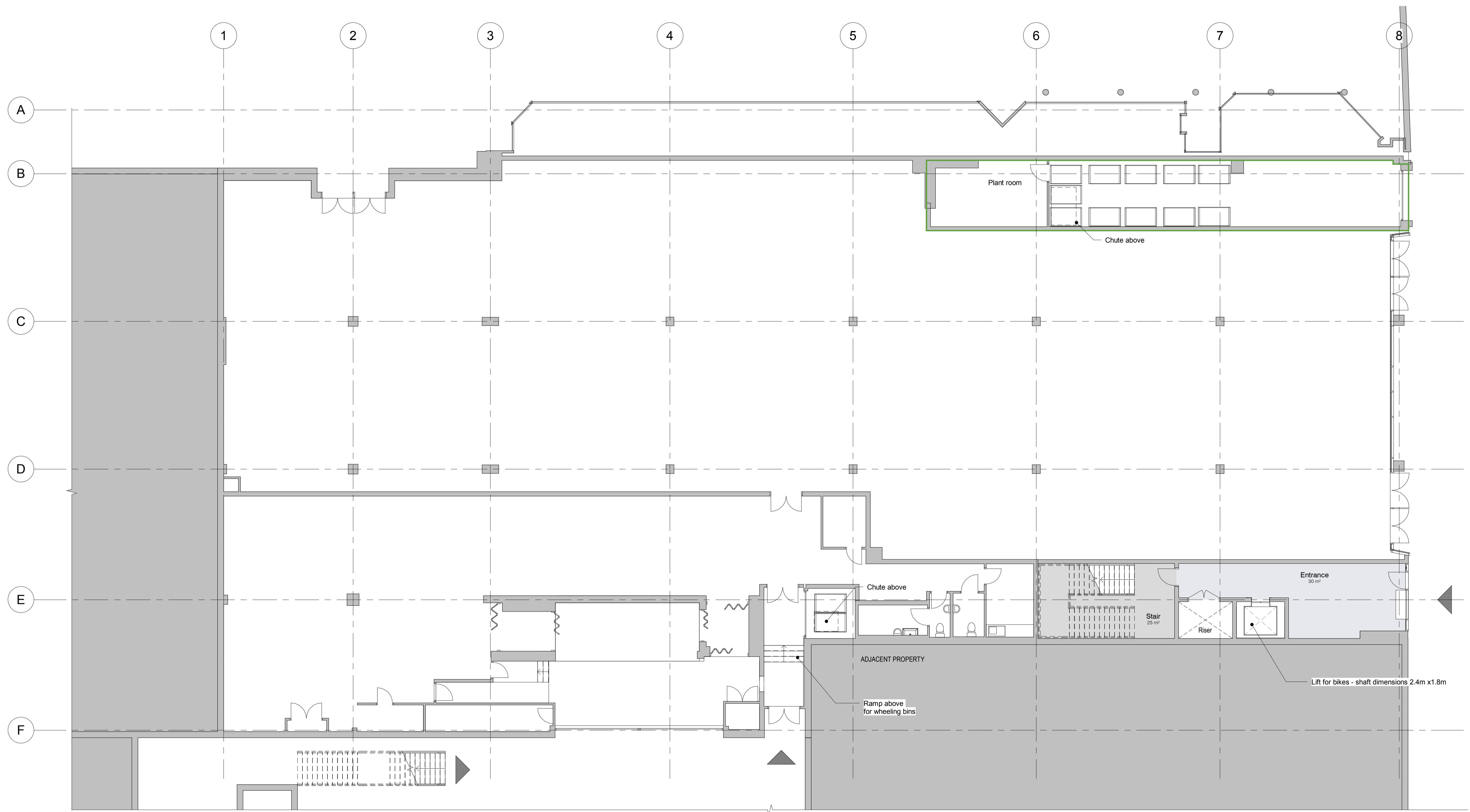
1. Level 0 - GA Proposed 1:100
